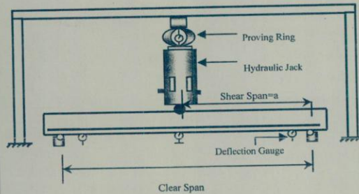
Fig. 4 Typical loading arrangement for testing of beams
