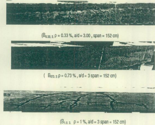
Fig. 5 Typical shear failure of beams without web reinforcement due to diagonal shear failure
