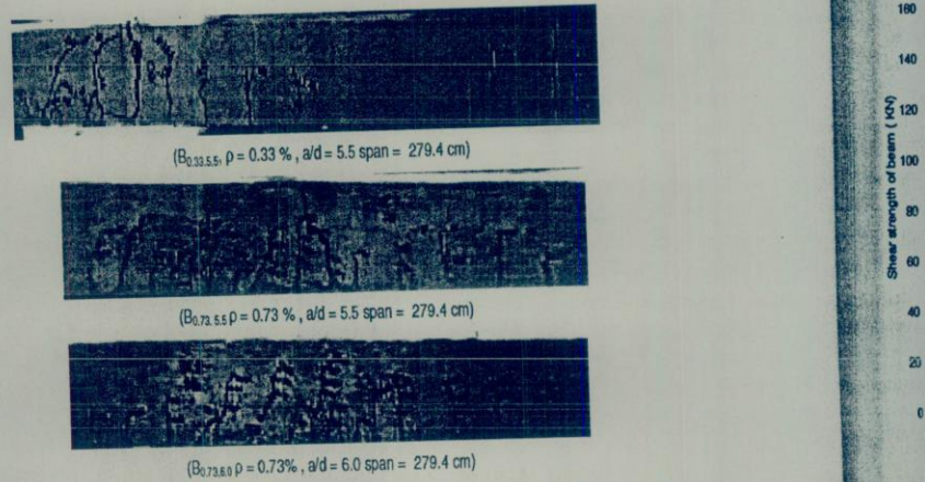
Fig. 6 Flexural shear failures of beams without web reinforcement for a/d > 5
