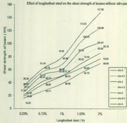
Fig. 8 Effect of longitudinal Steel ratio on the shear strength of concrete beams without stirrups for same value of a/d
