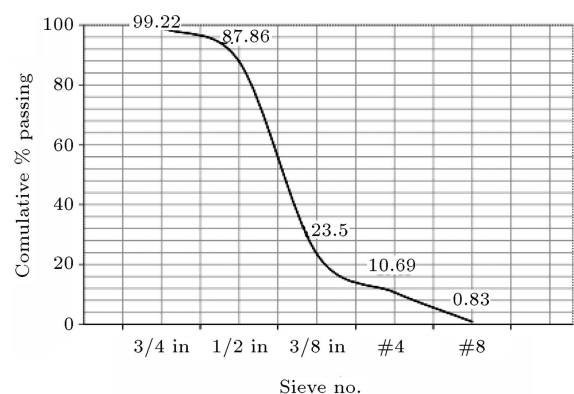
Figure 1. Gradation curve of crushed recycled aggregates collected from construction wastes.
