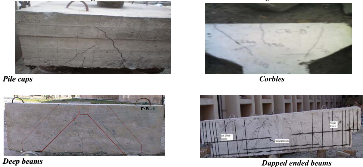
Fig.6 Typical failure modes of deep pile caps, corbelsl, deep beams and dapped ended beams.
